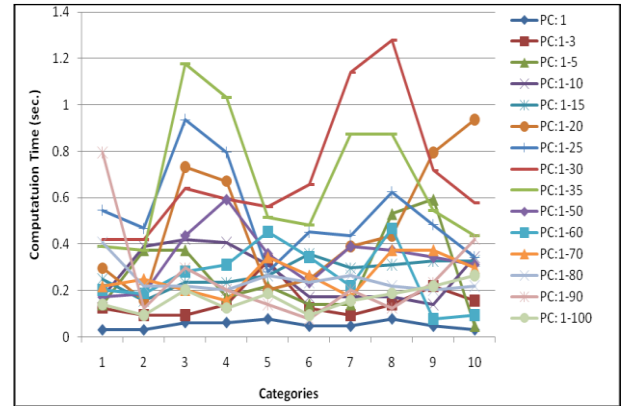
Fig. 16: Data formation, listing and labeling etc. time consumed by descriptors
