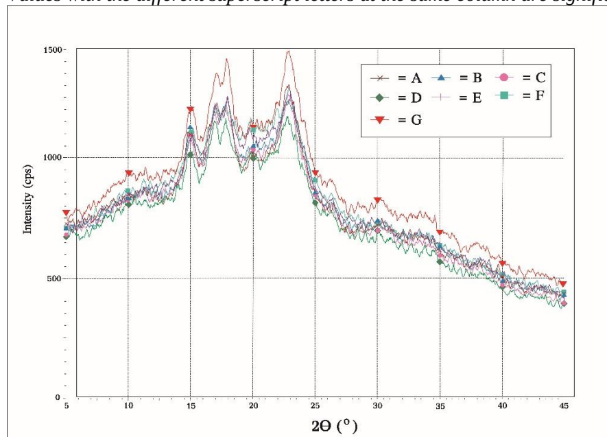
Figure-3. X-ray diffraction pattern of FCPF-based composite flour on various PG-autoclaving and cooling time (A = without treatment; B = PG autoclaving 15 min, cooling 24 h; C = PG autoclaving 15 min, cooling 48 h; D = PG autoclaving 15 min, cooling 72 h; E = PG autoclaving 30 min, cooling 24 h; F = PG autoclaving 30 min, cooling 48 h; G = PG autoclaving 30 min, cooling 72 h).
