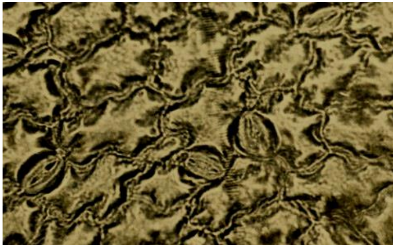
Fig. 5e. Two anisocytic stomata with common subsidiaries on ventral side of 7-day old cotyledon. 40 x 10 X.
