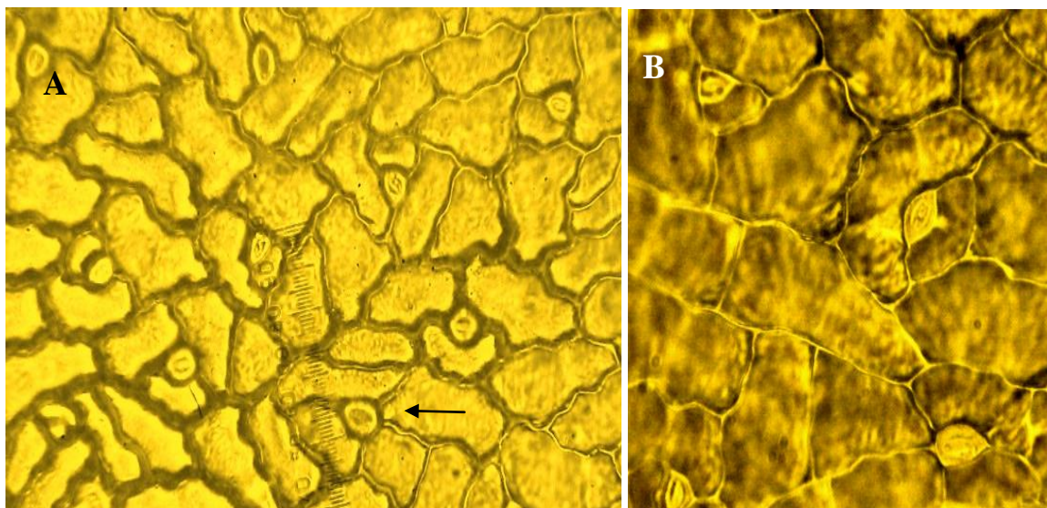
Fig. 9. Stomata of dorsal surface of leaflet of secondary leaf. Stomata are generally anisocytic, paracytic and staurocytic stomata (staurocytic stoma shown by an arrow). The anticlinal walls of the epidermal cells are straight, curvy to sinuous.
