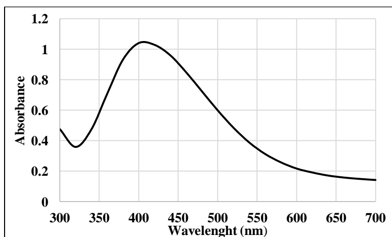
Fig. 2. UV-Visible absorption spectra of AV-AgNPs.
