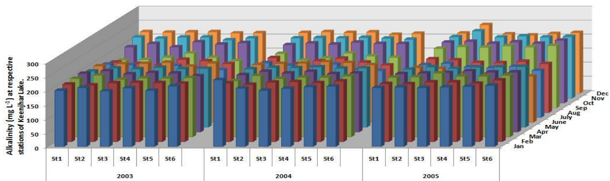
Figure 4. Alkalinity ( \text{mg L}^{-1} ) during 2003, 2004 and 2005 at respective stations from Keenjhar Lake.
