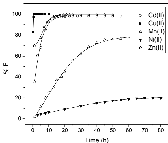
Figure 5. Extraction kinetics of metal ions.
