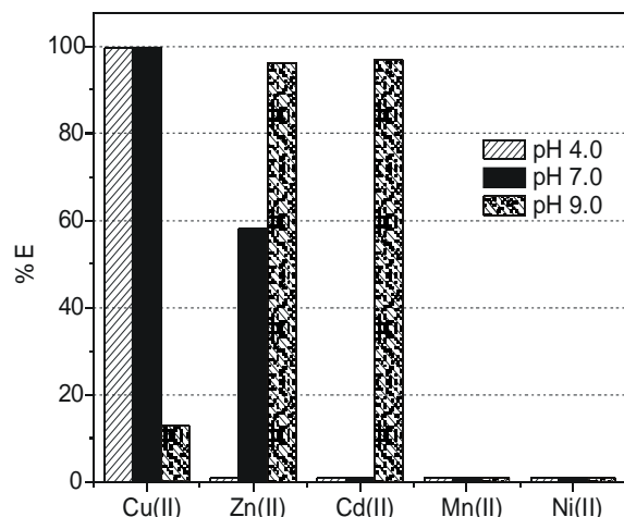
Figure 7. Extent of extraction as a function of pH
