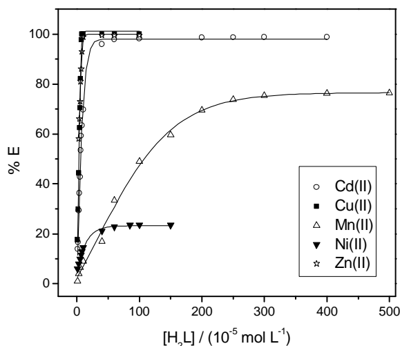
Figure 4. Maximum extraction capacity of metal ions.
