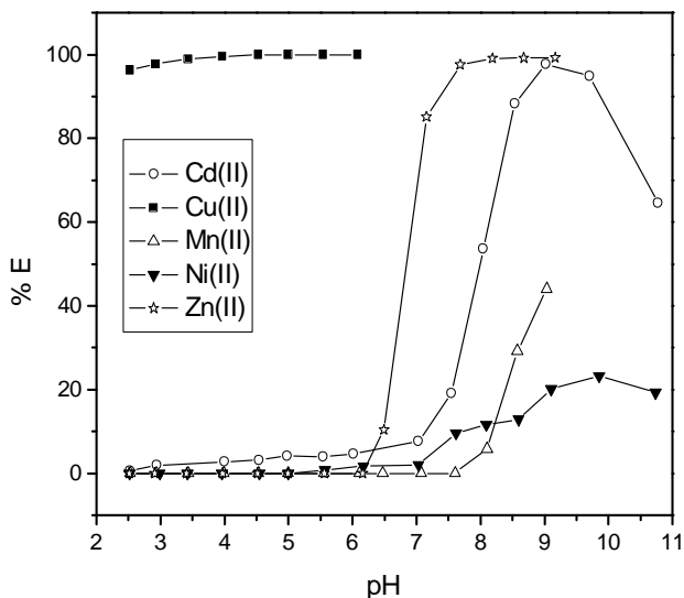
Figure 2. Effect of pH on the extraction of metal ions.
