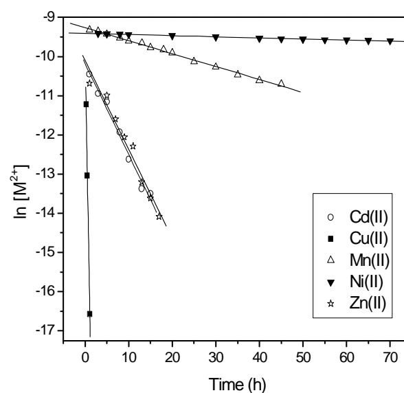
Figure 6. Pseudo-first-order kinetic model for the extraction of metal ions.
