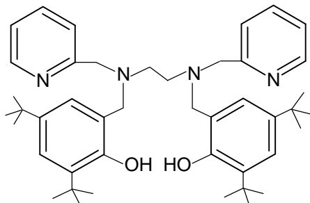
Figure 1. Chemical structure of H_2L ligand.
