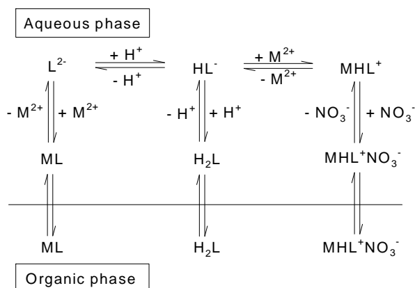
Figure 3. Chemical equilibria of the M^{2+} - H_2L - KNO_3 extraction systems.
