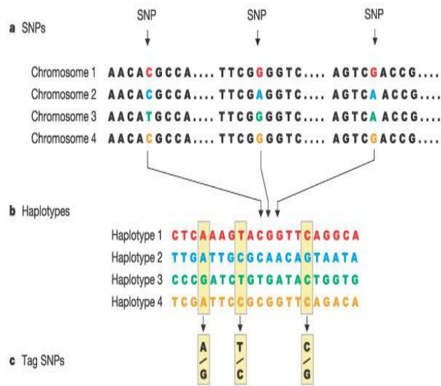
Fig. 2: Construction of the haplotypes
